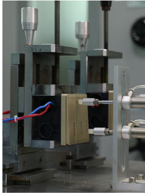
▲ Lifespan Test Machine
