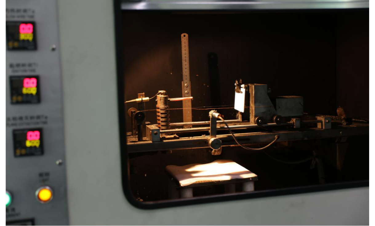
Glow-wire Test Machine ▲
